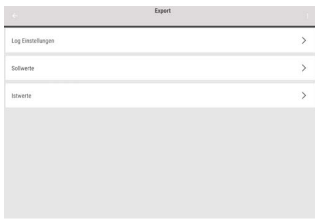
Abb. 20: Export
